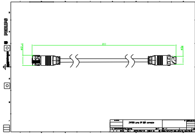
ZXP399 Jump 5P DMX connector (10 pcs)
